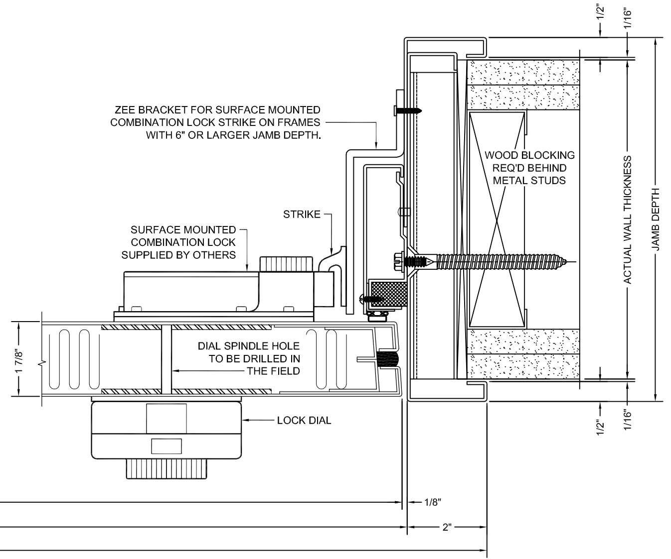
STRIKE JAMB SECTION
